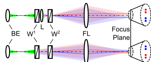
Fig. 27 Two-point beam propagation using a parallel beam arrangement (top) and a nonparallel beam arrangement (bottom).
