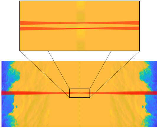
Fig. 39 Computational setup for estimating the effects of hypersonic turbulent boundary layers along a wind tunnel on a centerline measurement. Reproduced with permission from [106], ©2022, Optical Publishing Group.
