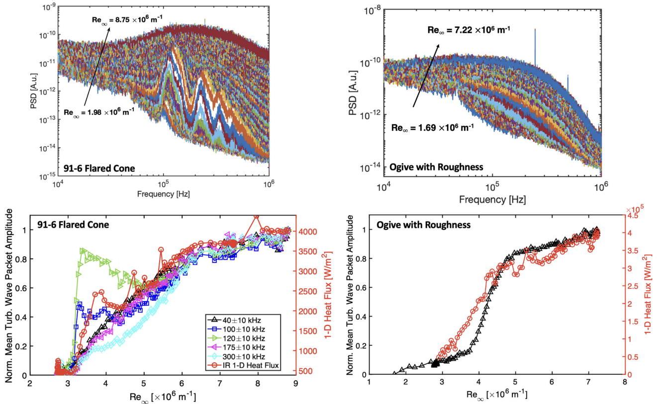
Fig. 29 Results from Siddiqui et al. [119] showing power spectra from FLDI in a transitional boundary layer and how the mean amplitude of density fluctuations in different frequency bands evolves in comparison to 1D heat flux determined from IR thermography. Reproduced with permission from [119], ©2023, Springer-Verlag GmbH.
