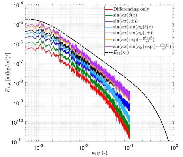
Fig. 28 Results from Hameed and Parziale [99] showing 1D energy spectra of the density fluctuations for an experiment performed with a round turbulent jet, corrected by transfer functions for disturbance fields as labeled. Reproduced with permission from [99], ©2022, AIAA.
