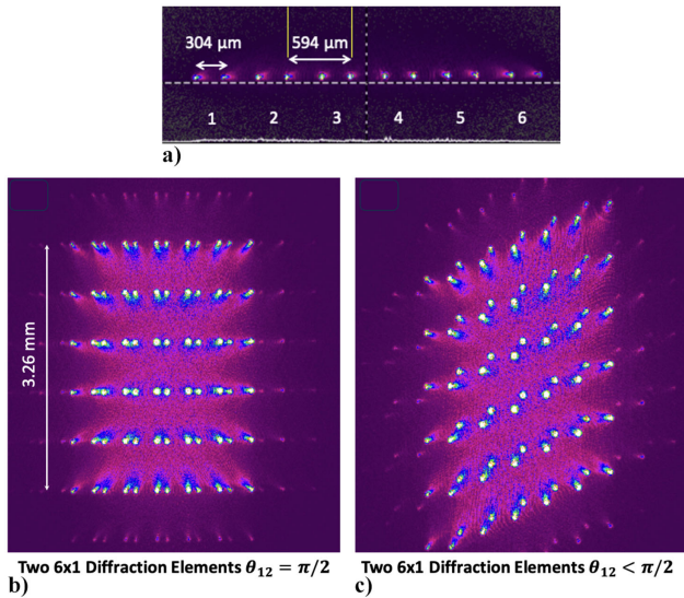
Fig. 23 Example arrays of FLDI beam pairs created using diffractive optics [81]. a) A linear distribution of six beam pairs from a single diffractive optic ( 6 \times 1 ). b) A 2D array of FLDI beam pairs and c) a parallelgram arrangement created by two diffractive optics. Reproduced from [81] with permission of the authors.
