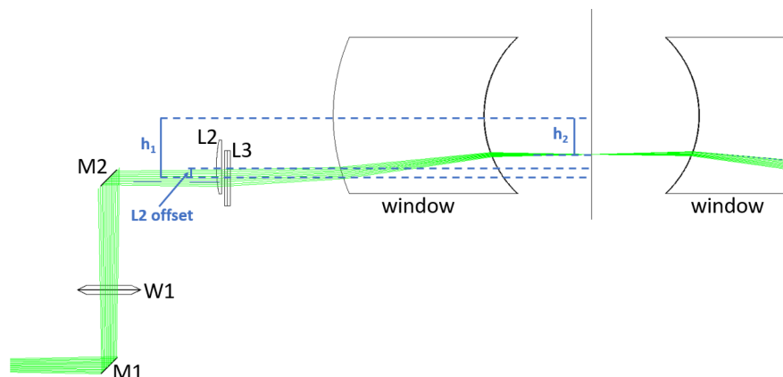
Fig. 45 Simulation of FLDI beams made in Zemax TM to design an optical setup compatible with contoured tunnel windows [49]. Reproduced with permission from [49], ©2021, AIAA.
