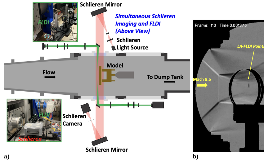
Fig. 43 a) An illustration of the setup used by Dean et al. [87] showing a Z-type setup of FLDI and mirror-based schlieren imaging, using conventional schlieren mirrors rather than FLDI lenses. b) An image from the experiment showing several FLDI beams in a schlieren image, which appear as dark spots due to postprocessing.
