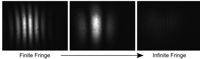
Fig. 8 Images of the fringe pattern produced as the recombination Wollaston prism is moved along the optical axis. Note that the phase of the fringe will determine whether the infinite fringe appears totally dark, totally bright, or somewhere in between.
