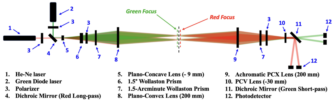
Fig. 47 The optical layout used by Webber et al. [71] for a multidepth FLDI that produces additional points along the beam axis. Reproduced with permission from [71], ©2024, Optica Publishing Group.
