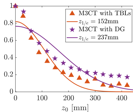
b) Response to 64 mm square test section of M3CT, \theta_d = 0.014
