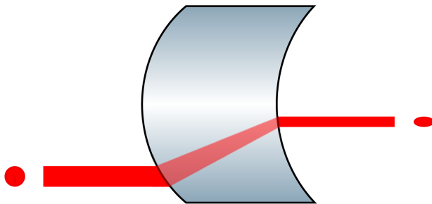
Fig. 44 Illustration of two effects a contoured window has on a circular beam. The beam is displaced in relative position, and its profile is no longer Gaussian after passing through the contoured window, which acts like a cylindrical lens that transforms the circular beam into an elliptical beam.
