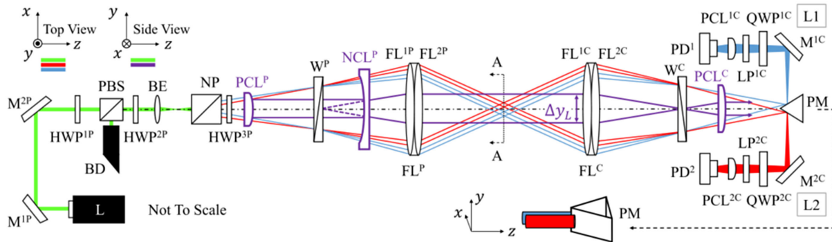
Fig. 21 Schematic of a two-line FLDI system used for multipoint sampling of a flowfield. The cylindrical optics allow for measurement along a line, and a Nomarski prism is used to make a two-line measurement. Reproduced with permission from [47], ©2020, Optica Publishing Group.
