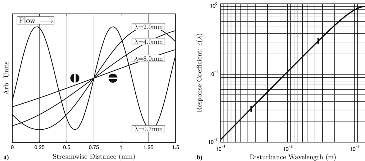
Fig. 5 a) Four sine waves representative of density disturbances of equal amplitude with wavelengths 0.7, 2, 4, and 8 mm, with two circles representing the beam polarized in the streamwise and spanwise directions, denoted by the horizontal and vertical lines through the circles, respectively. b) Plot of the response coefficient as a function of wavelength. The error bars here represent the error due to the beam spacing. Reproduced with permission from [20], ©2014, Springer-Verlag GmbH.
