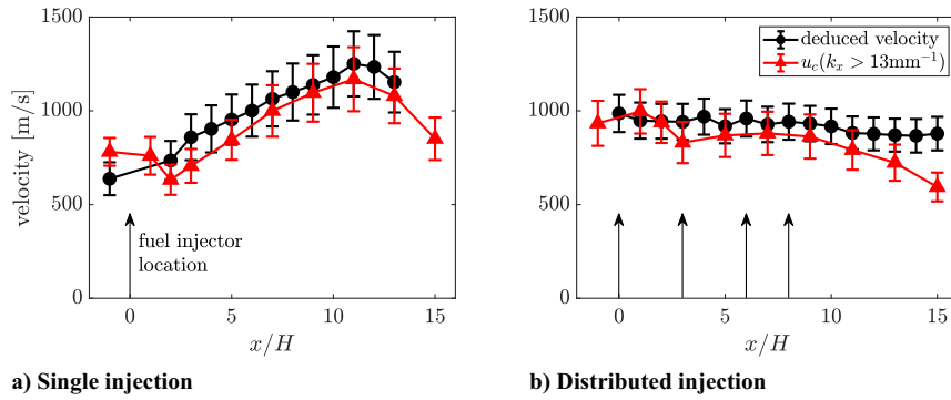
Fig. 35 Two-point FLDI axial velocity profiles, u_c , in a scramjet combustor [138]. “Deduced velocity” is found from a combination of pressure measurements, chemiluminescence, and quasi-1D flow analysis. Reproduced from [138] with permission from the authors.
