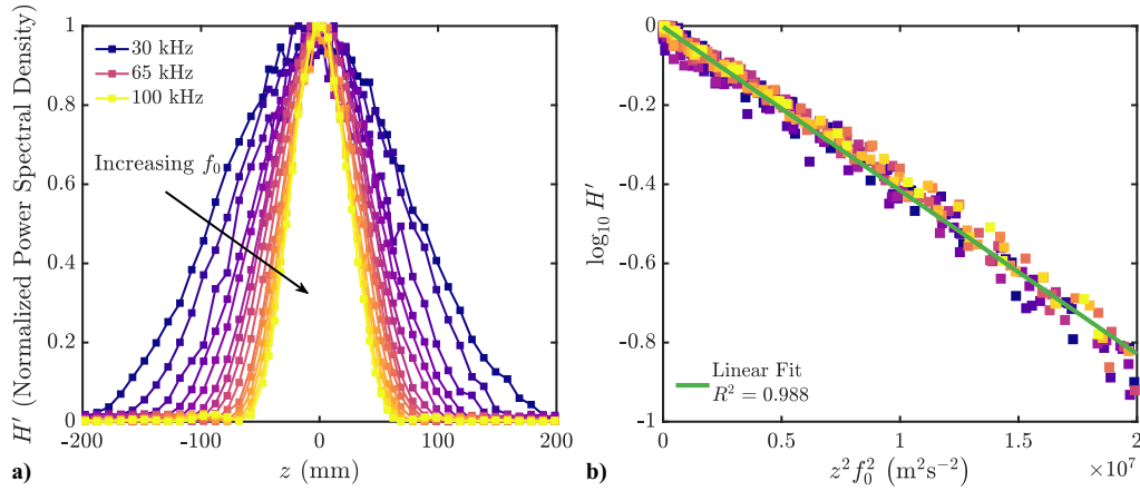
Fig. 18 Results of the ultrasonic beam experiments from Lawson et al. [104]. a) Drop-off in FLDI response moving away from the location of the foci at z = 0 . b) Same data as (a) but plotted using the variables suggested by the analytical transfer function model. Frequencies f_0 range from 30 to 100 kHz in 5 kHz increments. Reformatted using data from Lawson et al. [104], courtesy of J. M. Lawson.
