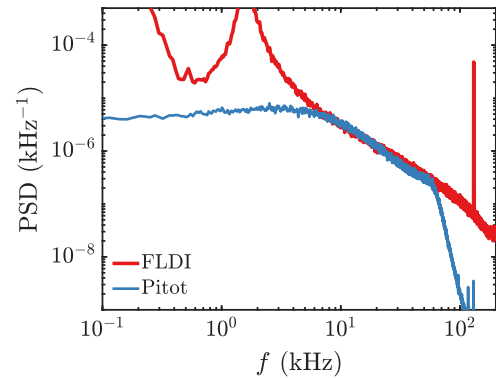
Fig. 20 Comparison of converted FLDI and Pitot spectra of freestream disturbances in VKF Wind Tunnel D Run 183, M_\infty = 5 . Reformatted using data from Lawson et al. [105], courtesy of J. M. Lawson.
