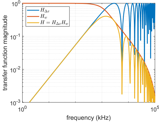
Fig. 37 Example FLDI transfer functions with \Delta x = 150 \mu\text{m} , w_0 = 5 \mu\text{m} , \lambda_0 = 633 \text{ nm} , and u_c = 860 \text{ m/s} . Reproduced with permission from [111].
