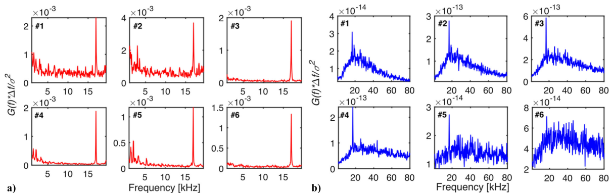
Fig. 24 Mach 1.5 jet screech frequencies measured at six points using the a) high-speed camera-based measurement method and the b) fiber-optic-coupled photodiode measurement method. Reproduced from [81] with permission of the authors.
