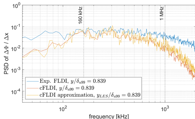
Fig. 40 PSDs comparing computed FLDI signal with experimental data for a hypersonic turbulent boundary layer. Reproduced with permission from [92].
