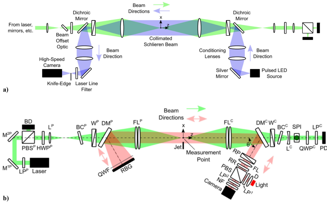
Fig. 41 Schematics of the a) collinear FLDI and conventional schlieren from Bathel et al. [28] and the b) collinear FLDI and self-aligned focusing schlieren from Weisberger and Bathel [52]. Reproduced with permission from [28], ©2021, IOP Publishing and [52], ©2023, Optica Publishing Group.
