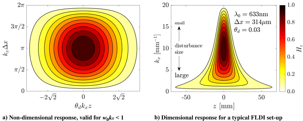
Fig. 12 FLDI sensitivity to flow-parallel sinusoidal waves.
