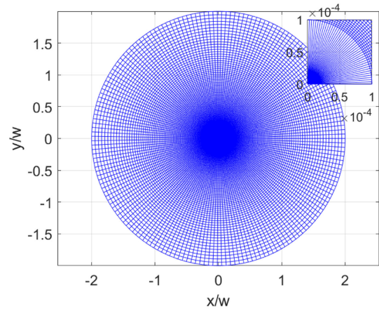
Fig. 36 Example polar coordinate FLDI beam profile grid with 180 azimuthally distributed points and 363 radially distributed points. Reproduced with permission from [109], ©2023, AIAA.
