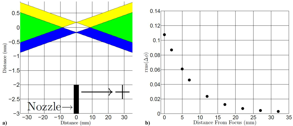
Fig. 3 a) Schematic of the small \text{CO}_2 nozzle and laser beam profile, with the arrow denoting the direction of nozzle traversal. The yellow- and blue-shaded areas denote where the laser is polarized either along the streamwise direction or normal to the page, respectively. The green-shaded region denotes the area where the two laser beams overlap. b) Results of the bench test, demonstrating the decrease in response of the FLDI with increasing distance from the tightly focused sensitive region. Reproduced from [19] with permission of the author.
