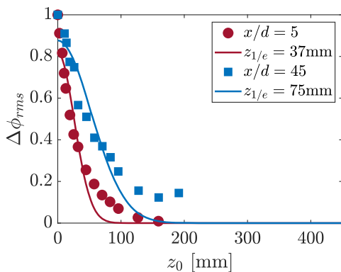
a) Response to 3 mm diameter turbulent jet, \theta_d = 0.029
