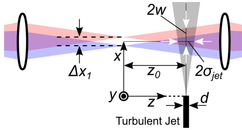
Fig. 13 Schematic of turbulent jet experiment to investigate optical-axis sensitivity.
