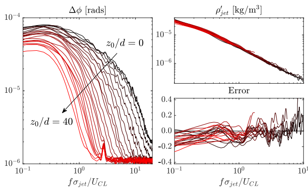
Fig. 19 Optical-axis spectral response to a turbulent jet, d = 3\text{ mm} and x/d = 25 ; \rho'_{jet} is obtained by dividing \Delta\phi by the transfer function described by Eqs. (20) and (21). Data replotted from Ceruzzi and Cadou [75].
