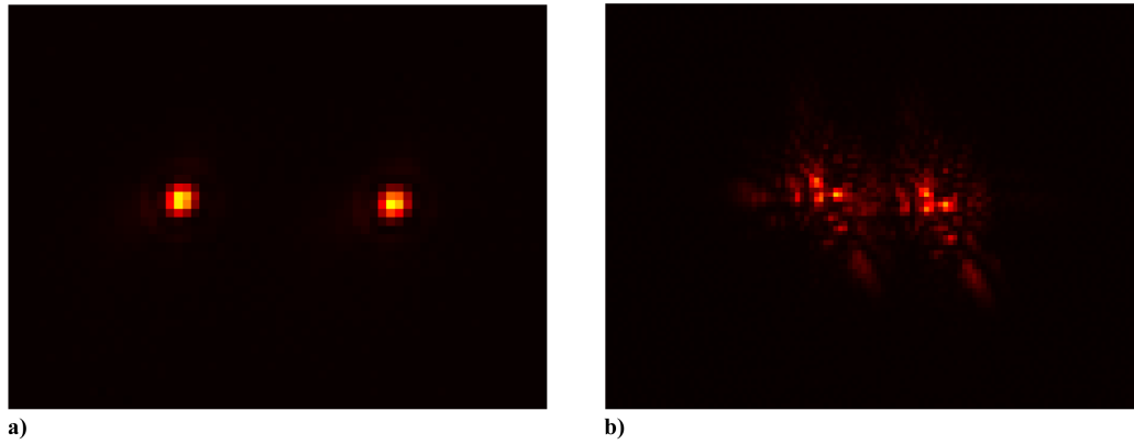
Fig. 46 FLDI beam foci for the a) traditional setup (without any windows) and b) the BAM6QT setup (with the Plexiglas contoured windows). Reproduced with permission from [49], ©2021, AIAA.
