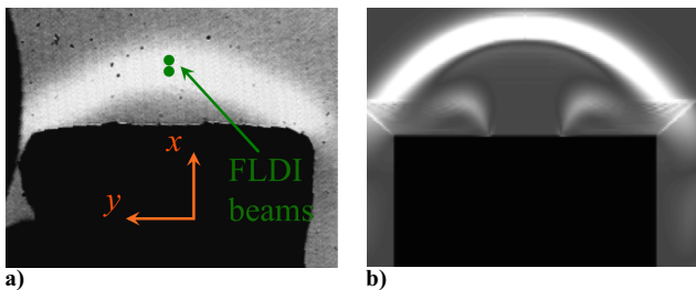
Fig. 16 a) Schlieren image of the argon jet in the x - y plane. The top of the jet is about 15 mm from the chamber exit and is observed to be uniform across the jet cross section, temporally stable, and laminar. b) Pseudo-schlieren image of the argon jet showing the vertical gradient in density for comparison with the experiment. Reproduced with permission from [96], ©2015, Optica Publishing Group.
