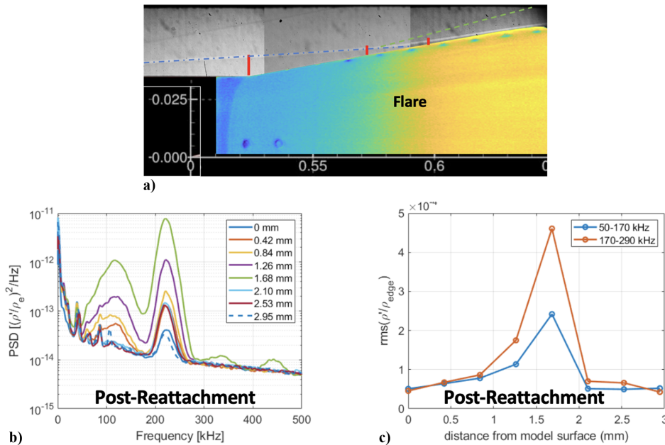
Fig. 30 Results from Benitez [132] showing fluctuation spectra and RMS magnitudes from FLDI measurements at different wall-normal positions in the reattached boundary layer on a cone-cylinder-flare geometry in Mach 6 flow. Reproduced from [132] with permission of the author.
