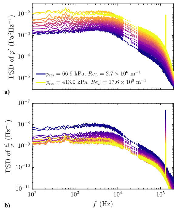
Fig. 32 Comparison of converted FLDI (>30kHz) and Pitot (<15kHz) spectra for all conditions within VFK Wind Tunnel D Run 186: M_\infty = 4 using the a) absolute pressure and b) relative pressure. Dashed lines indicate power-law extrapolations beyond the useful bandwidth of each instrument. Reformatted using data from Lawson et al. [105], courtesy of J. M. Lawson.
