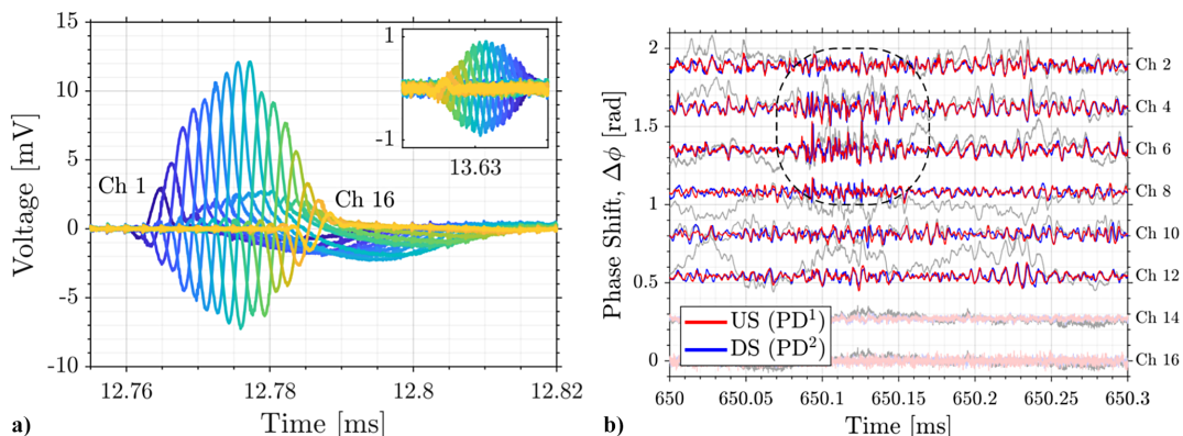
Fig. 22 a) Response of 16 channels to a traveling shock along major axis of beam. b) Flat-plate boundary-layer wall-normal measurement with second-mode wave packet outlined in dashed black, with upstream (US) and downstream (DS) lines identified. Reproduced with permission from [47], ©2020, Optica Publishing Group.
