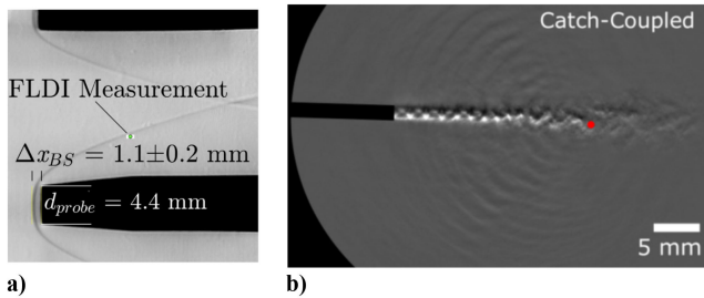
Fig. 42 a) An image from Bathel et al. [28] showing a conventional schlieren image acquired through the FLDI system lenses per the setup in Fig. 41a. The image was taken in Mach 6 flow conditions in a NASA facility. b) Image from Weisberger and Bathel [52] of self-aligned focusing schlieren image of a compressed air jet with FLDI measurement point identified with red dot. Reproduced with permission from [28], ©2021, IOP Publishing and [52], ©2023, Optica Publishing Group.
