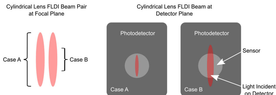
Fig. 10 A cylindrical lens FLDI setup with all light focused on detector, case A, will have contributions from the entire beam, resulting in spatial averaging along the major axis of the beam at the focal plane. If only a portion of the beam is used, case B, the spatial averaging is limited.
