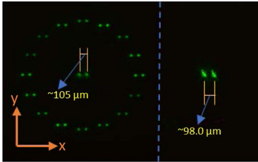
Fig. 26 FLDI beam array in the shape of a circular ring with a central point, demonstrating arbitrary beam array creation from the SLM [78]. Reproduced with permission from [78], ©2023, Optica Publishing Group.
