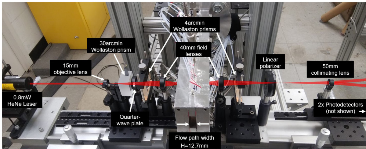
Fig. 34 Photograph of two-point FLDI probing a scramjet combustor at UMD's propulsion research lab [138]. Reproduced from [138] with permission from the authors.
