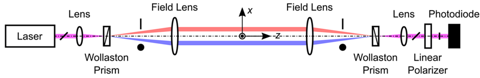
Fig. 1 Schematic of a nonfocusing laser differential interferometer (LDI), with pitch side of instrument on the left and catch side on the right.
