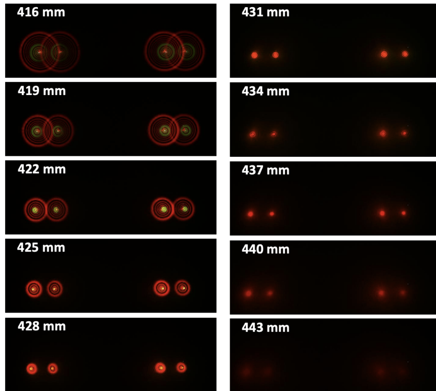
Fig. 48 Image montage showing multiple focal points along the optical axis, with lasers operating at 532 nm (green) and 632 nm (red) [71]. Reproduced with permission from [71], ©2024, Optica Publishing Group.
