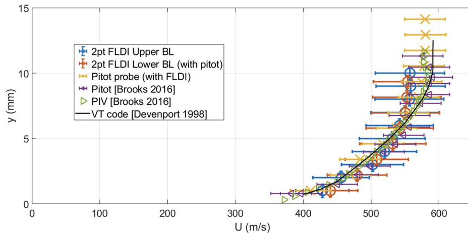
Fig. 31 A plot of a Mach 2.7 turbulent boundary-layer velocity profile obtained from FLDI by Ceruzzi et al. [72] with comparison to various other methods and computations. Reproduced from [72] with permission of the authors.
