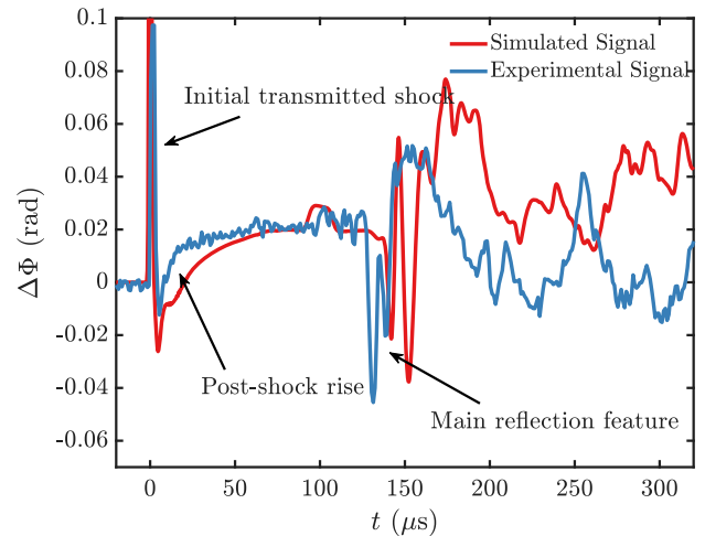
Fig. 38 Comparison between experimental data and a coupled AMROC/FLDI simulation of the shock reflection flowfield in HET. Reformatted using data from Lawson and Austin [108], courtesy of J. M. Lawson.
