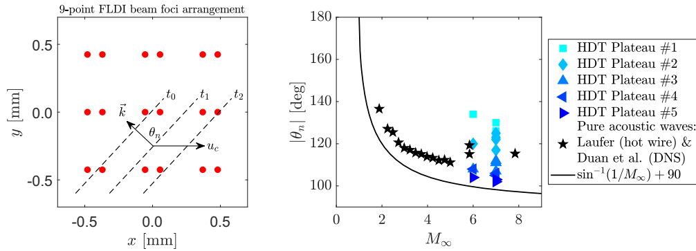
Fig. 33 Freestream wave inclination angles in the University of Oxford's High Density Tunnel (HDT) measured using cross-correlation between multipoint FLDI probes. The flat-plate data from Laufer [136] and Duan et al. [137] have been adjusted by 7 deg to account for the inclination angle of the nozzle where the waves in the HDT test section are expected to originate. Reproduced from [112] with permission from the authors.
