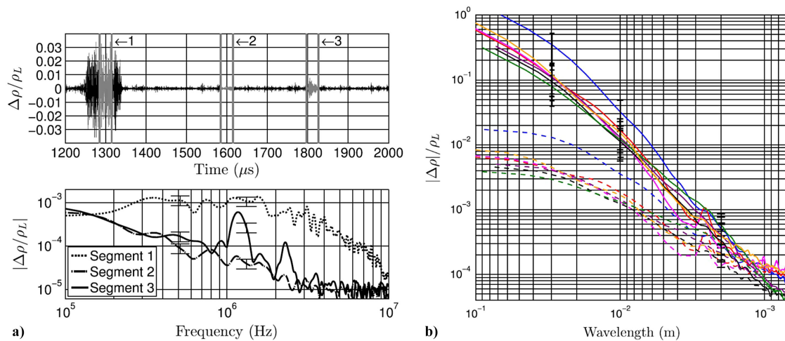
Fig. 4 a) FLDI results from shot 2702: the processed response (top) and spectral response from the three chosen segments (bottom). Reproduced with permission from [18], ©2013, AIAA. b) Wavelength spectrum of tunnel noise time traces for a range of T5 run conditions. The lower-amplitude data (dashed lines) have not been corrected for the sensitivity of the FLDI technique to wavelength, while the higher-amplitude data (solid lines) have been corrected for the sensitivity of the FLDI technique to wavelength. Reproduced with permission from [20], ©2014, Springer-Verlag GmbH.
