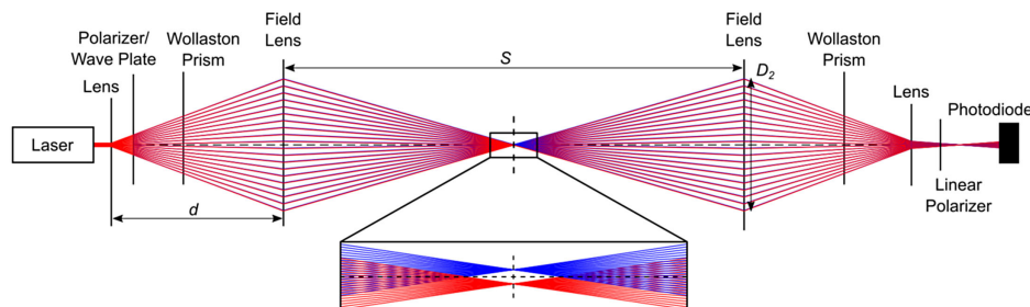
Fig. 7 The optical layout and ray trace of a basic FLDI system, including the following components: 1) laser, 2) plano-concave lens for beam expansion, 3) polarizer or half-wave plate, 4) Wollaston prism, 5) plano-convex field lenses, 6) secondary plano-concave lens, and 7) photodetector.
