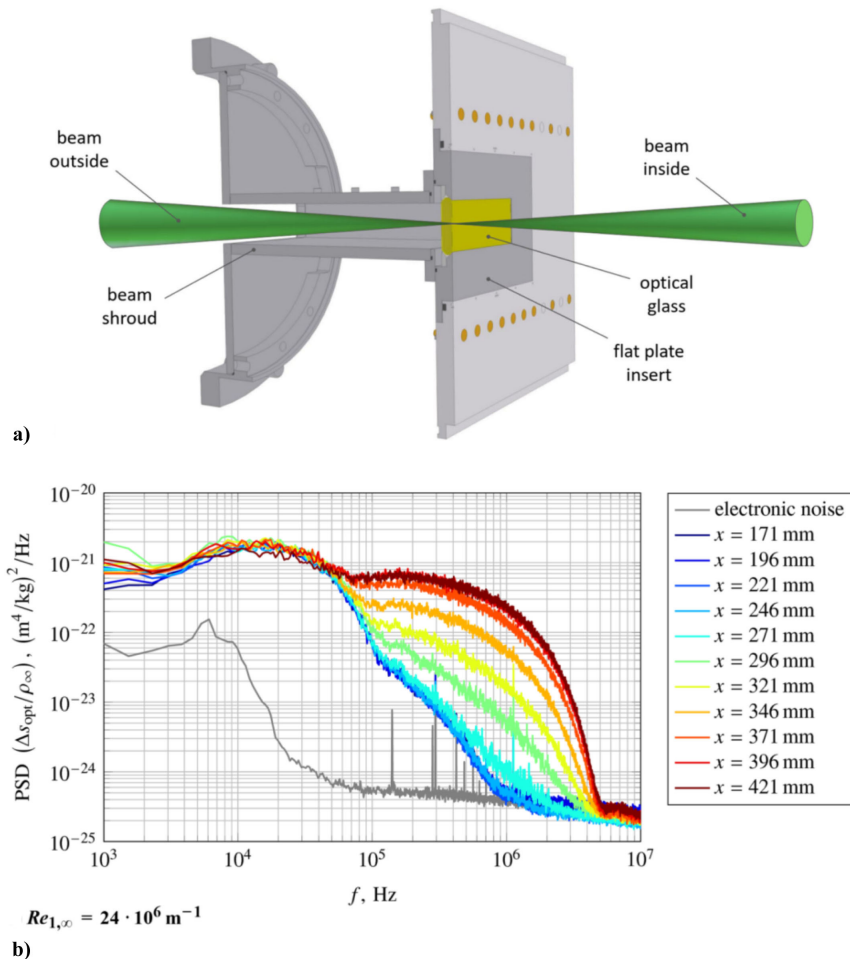
Fig. 49 a) Schematic of FLDI system projecting through the model sting from Lunte and Schüleln [37,39]. b) Power spectral density plot for a single Reynolds number of streamwise measurement positions. Reproduced from [39] with permission, ©2024, Lunte and Schüleln.
